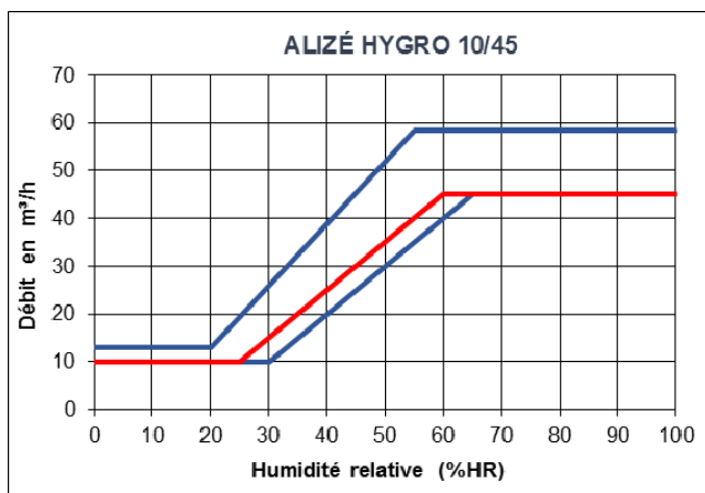
Figure 26 – HBO3 – ALIZÉ HYGRO 10-45 (25-60%HR)
