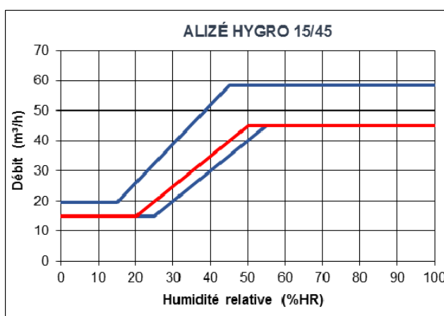
Figure 27 – HBO4 – ALIZÉ HYGRO 15-45 (20-50%HR)
