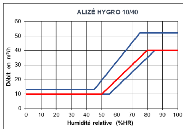
Figure 25 – HBO2 – ALIZÉ HYGRO 10-40 (50-80%HR)
