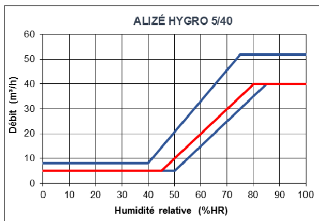
Figure 24 – HBO1 – ALIZÉ HYGRO 5-40 (45-80%HR)
